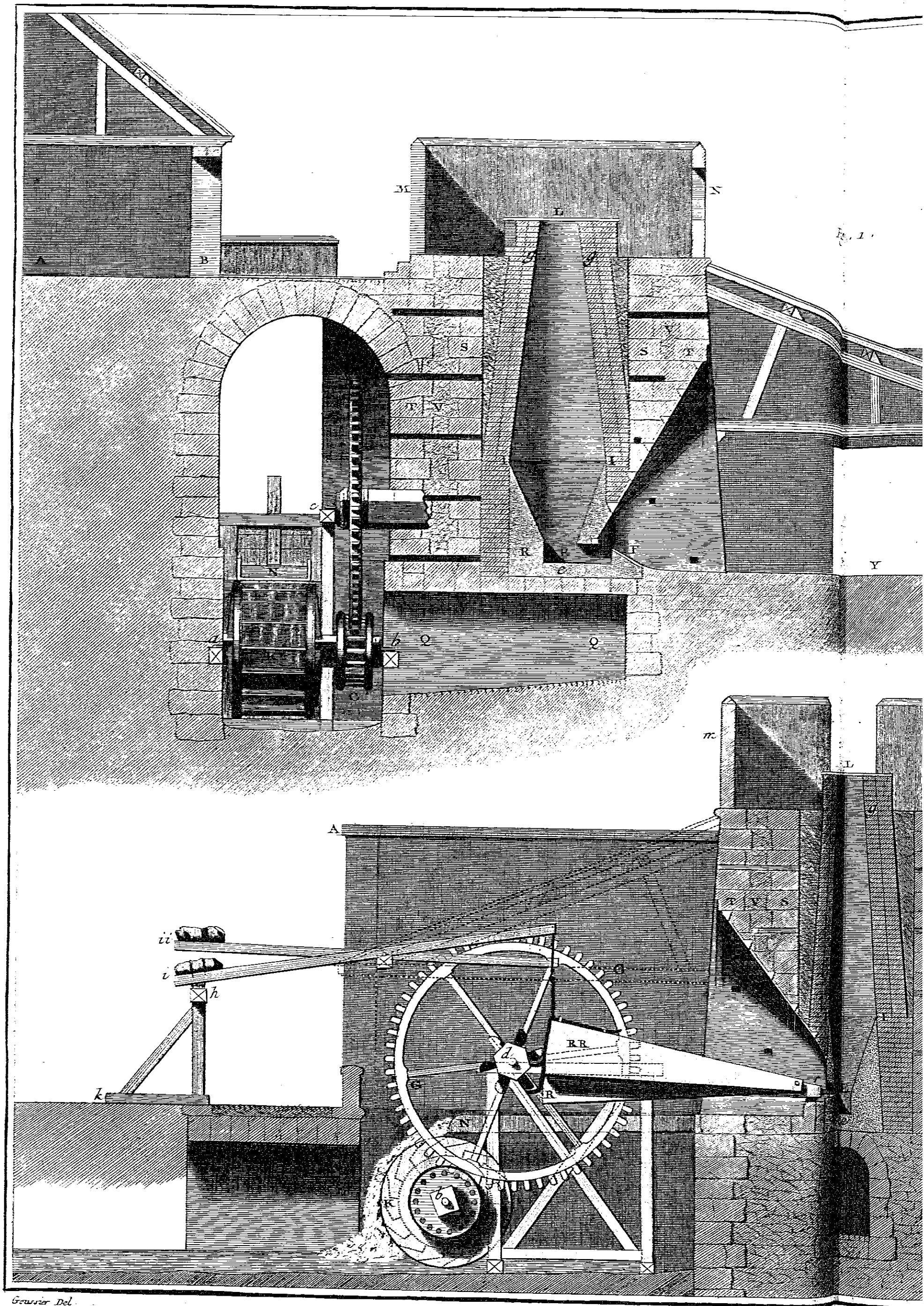
Forges, 3 e Section. Coup e d'un Four
