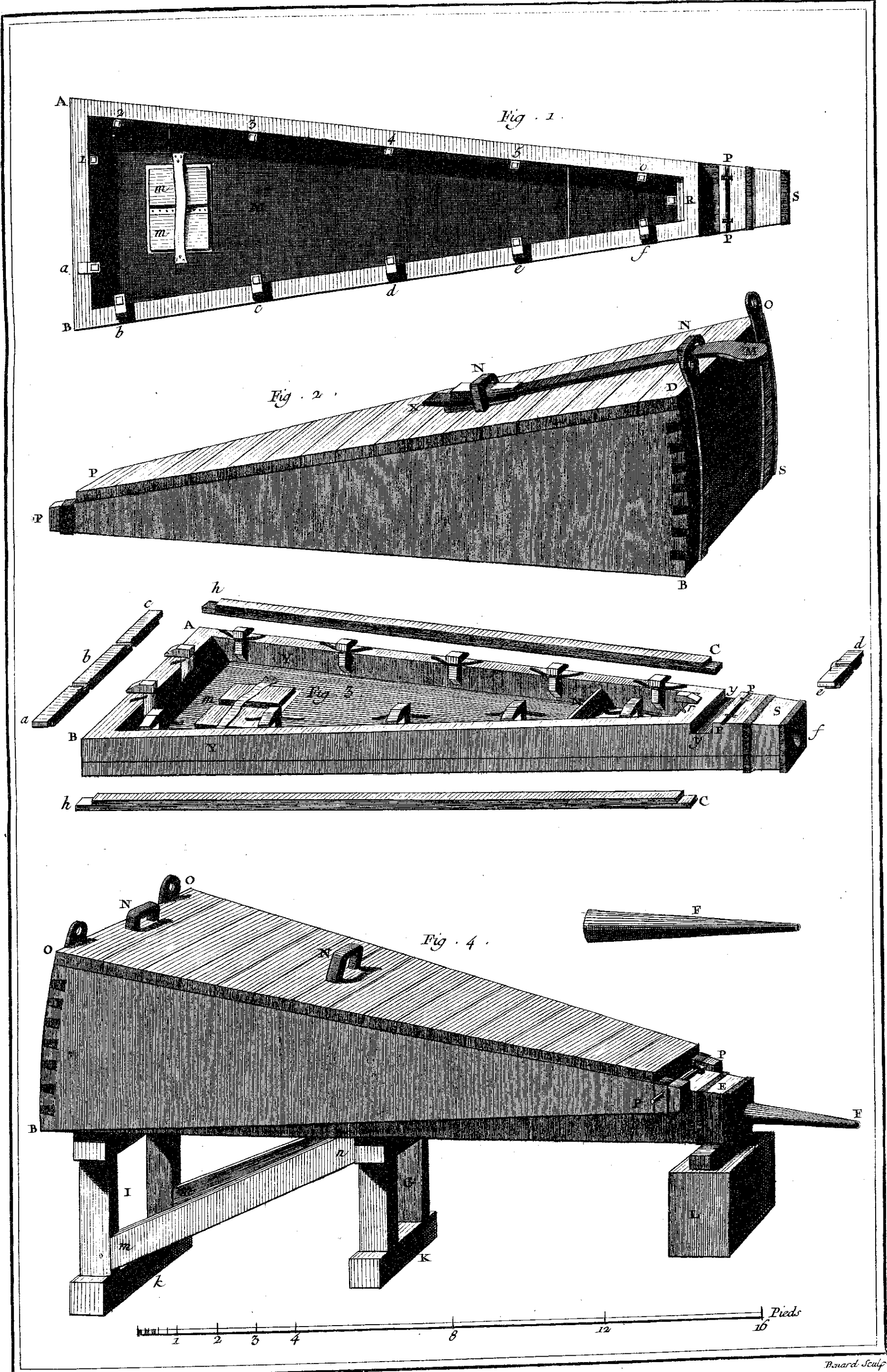
Forges, 2 e Section, Fourneaux à Fer, Soufflets.
